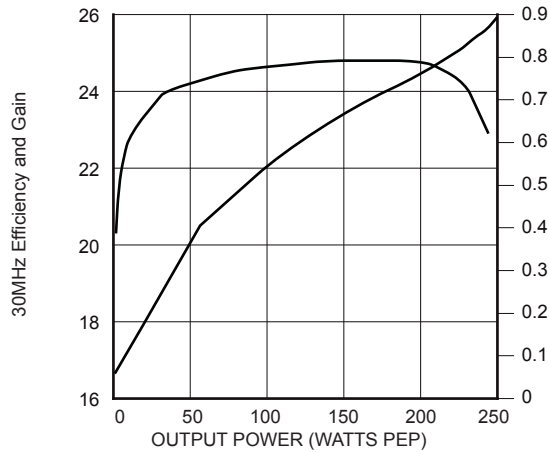
Figure 6. Gain and Efficiency vs P_{out}
