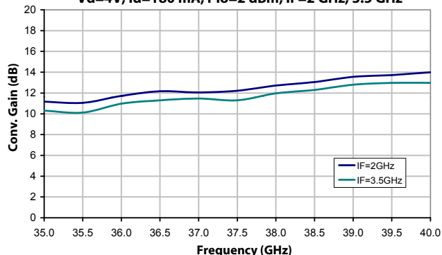
XR1008-QB: LSB Conversion Gain vs Frequency Vd=4V, Id=180 mA, Plo=2 dBm, IF=2 GHz, 3.5 GHz
